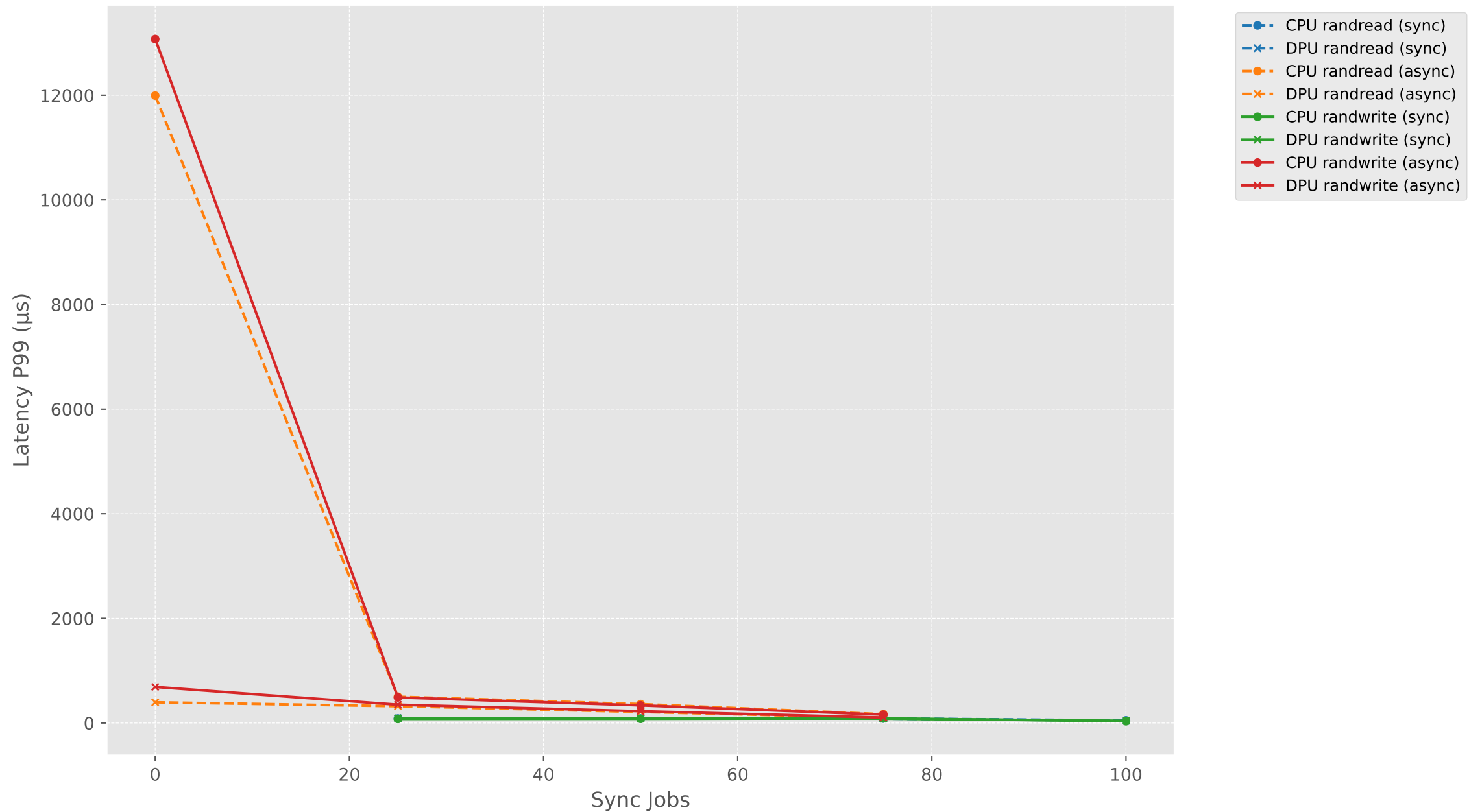
Latency P99 vs Sync Jobs (mixed) - RAND (CPU vs DPU)
